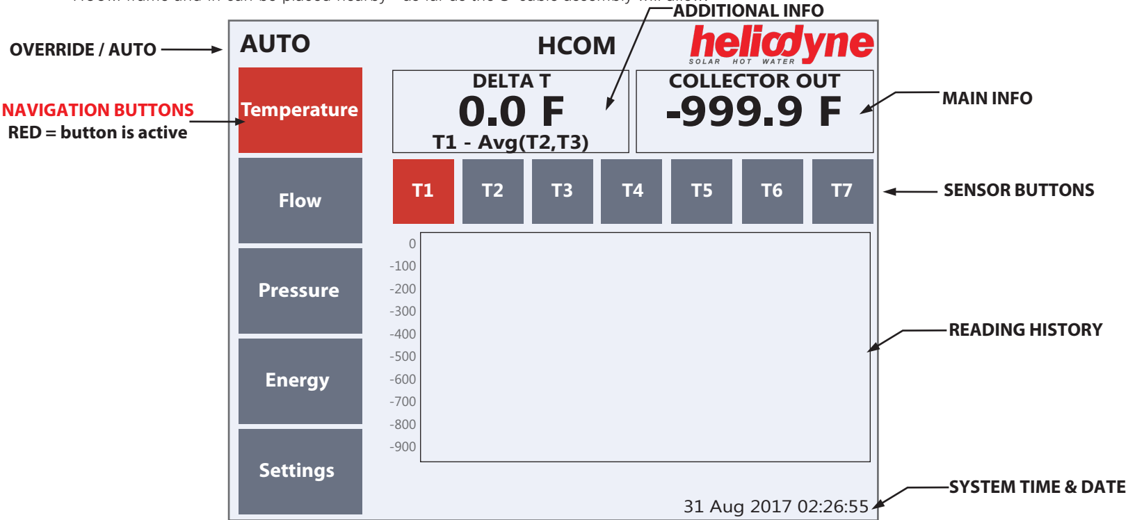
Figure 1.6-1: Display Navigation
