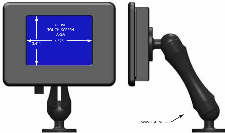
Figure 1.6.2-1: Display Dimensions
